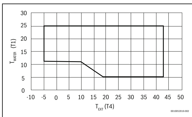
11. ábra CS2000AWF 4-6 R-S, CS2000AWF 8-10 R-S, CS2000AWF 12-16 R-S/T
